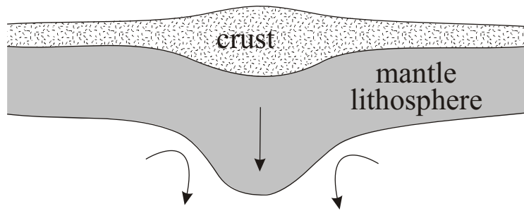
(a) gravitational (RT) instability
